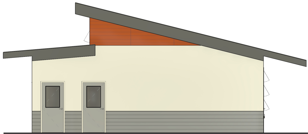
NORTH ELEVATION
